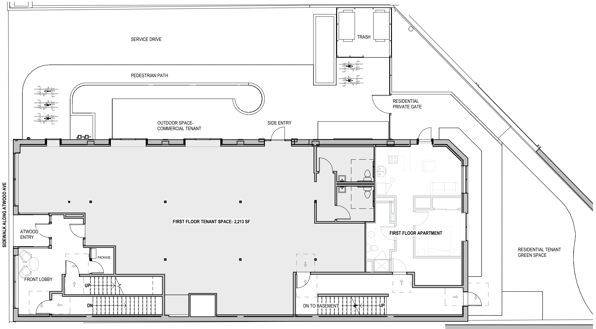
1 FIRST FLOOR TENANT SPACE 1/8" = 1'-0"
